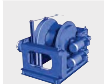
Mooring winches SRM integrated gears electric or hydraulic drive Load range 18.000-36.000 kg
